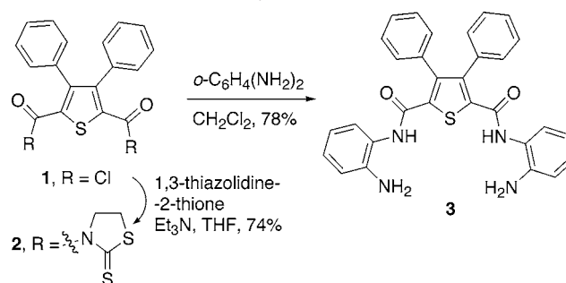
Scheme 1. Synthesis of Precursor 3
