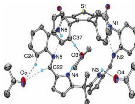
Figure 1. ORTEP-POVray rendered view of 6 showing three bound acetone molecules. Most hydrogen atoms have been removed for clarity. Thermal ellipsoids are scaled to the 50% probability level.
