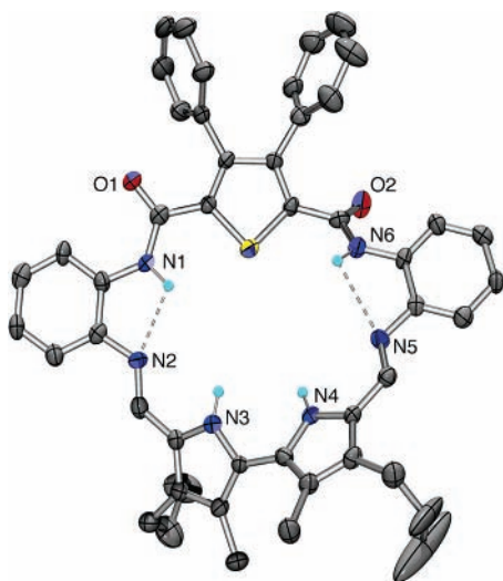
Figure 2. ORTEP-POVray rendered view of 7 . Most hydrogen atoms have been removed for clarity. Thermal ellipsoids are scaled to the 50% probability level.
